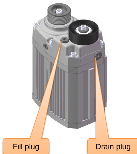
Supercharger without Sight glass
