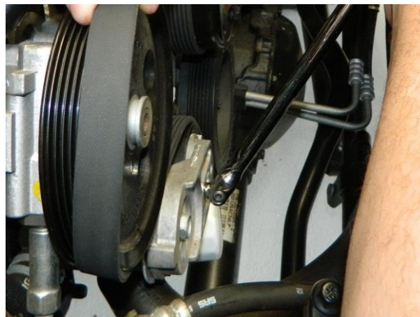
Supercharger without Sight glass
